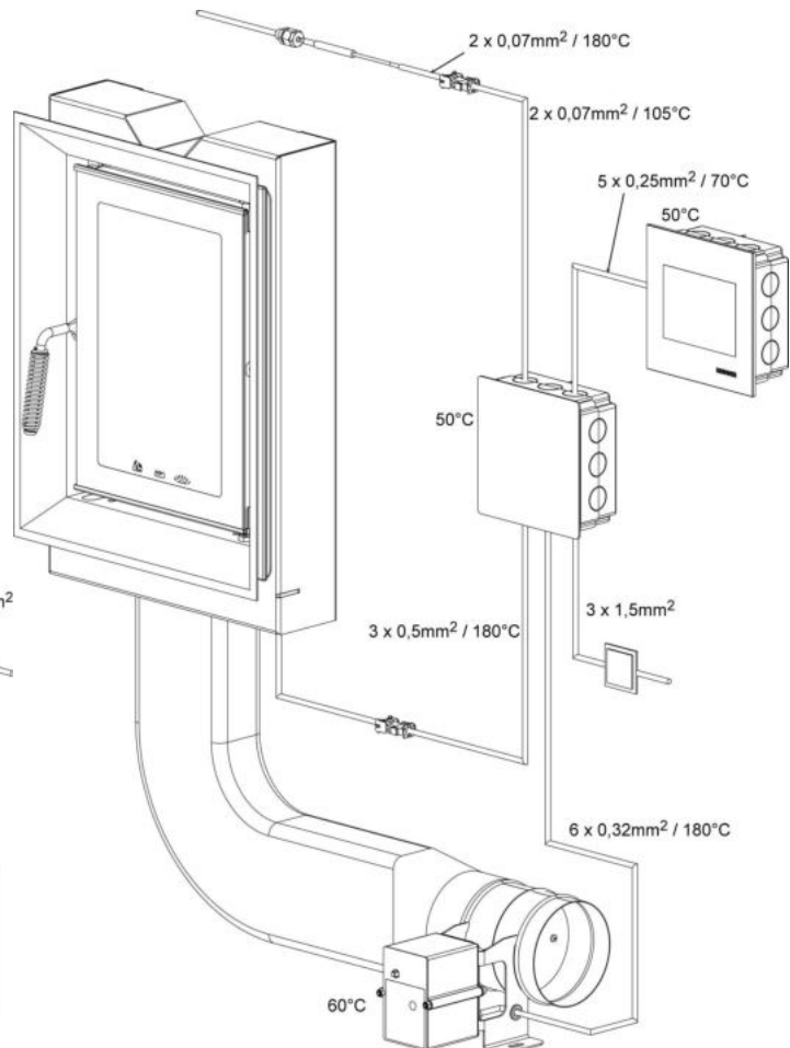
Im. 3: Schematic layout of EOS
